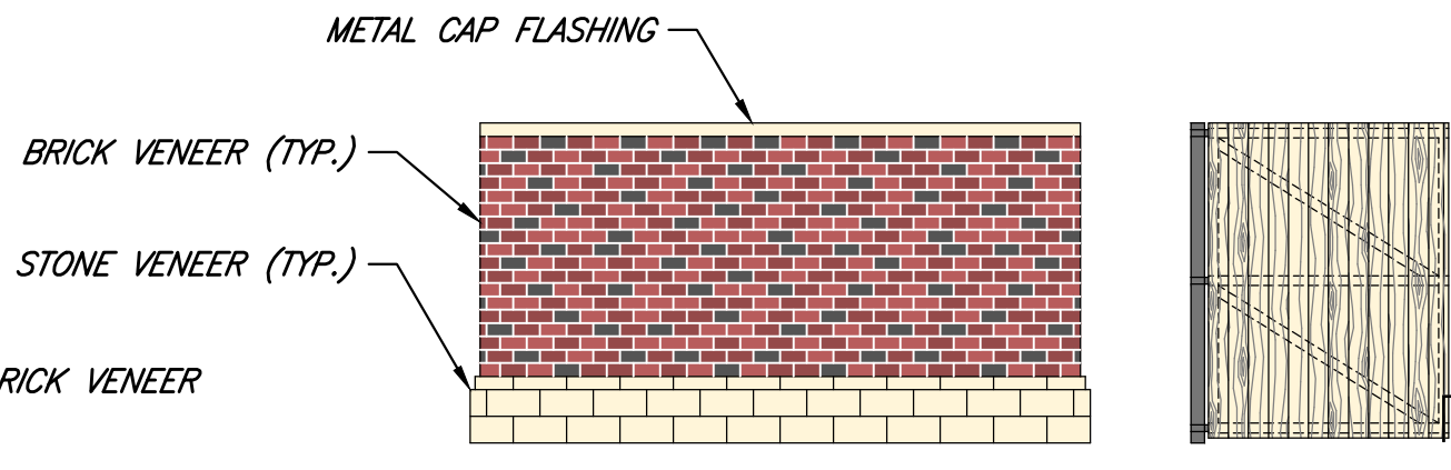
DUMPSTER ENCLOSURE ELEVATION 3/16" = 1'-0"
